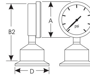
Bottom Mount
