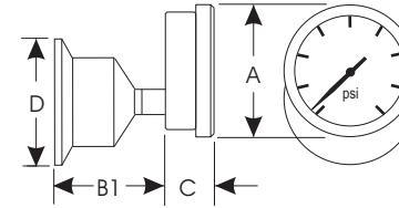
Back Mount
